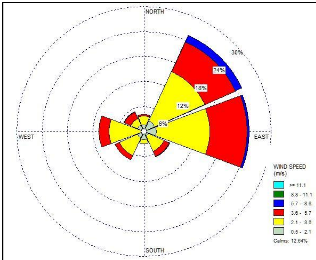
Figure Error! No text of specified style in document.-1 Wind rose diagram for the Study Period (October 2021-December 2021)
