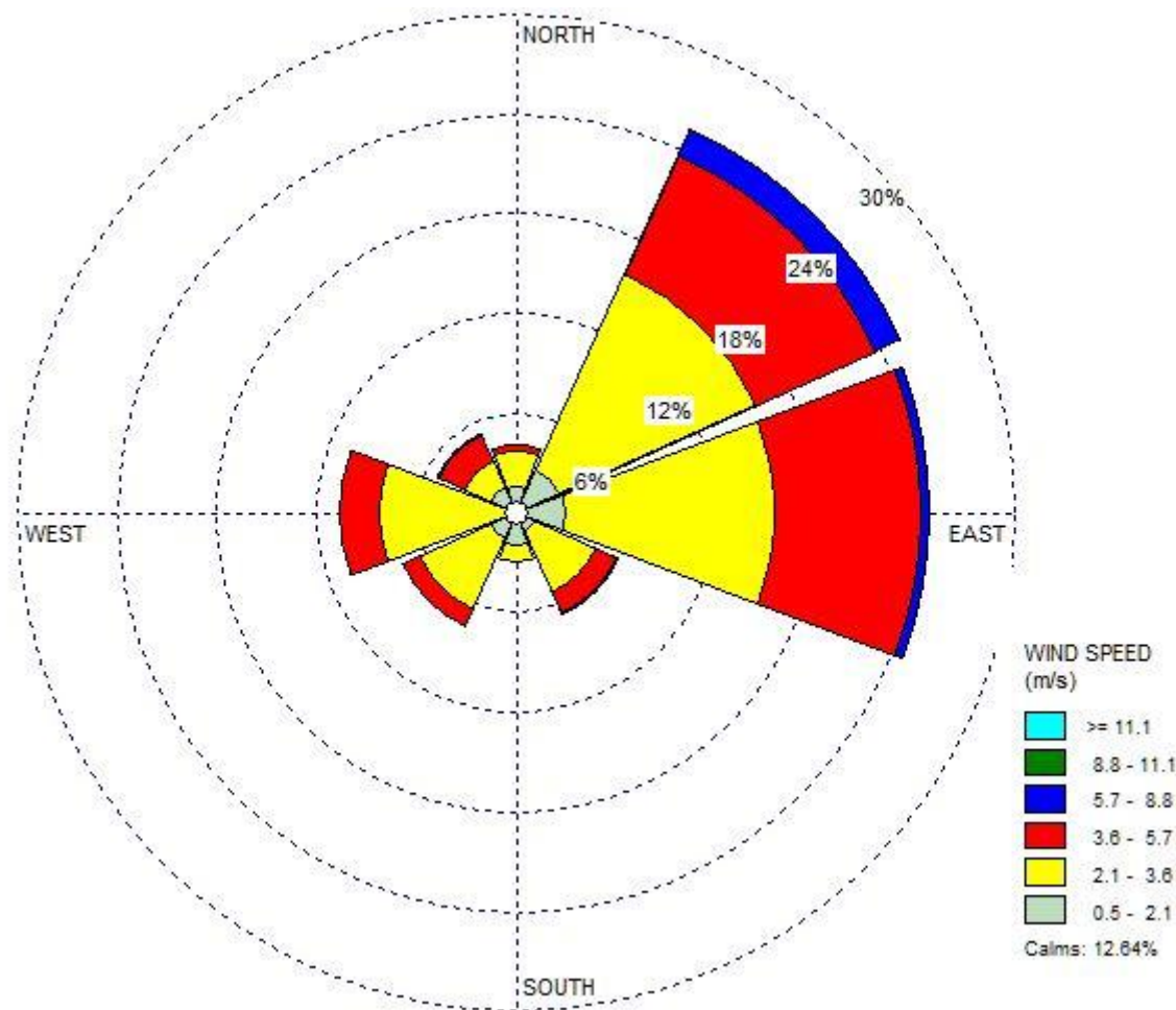
Figure- 1 Wind rose diagram for the Study Period (October 2021-December 2021)
