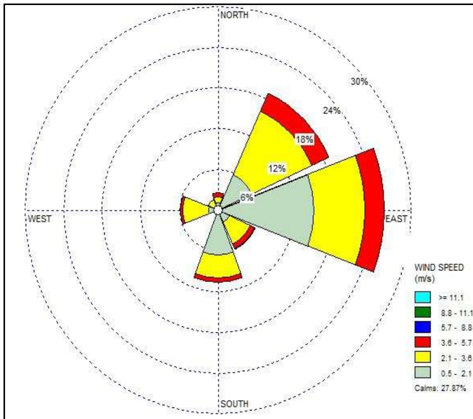
Figure 0-1 Wind rose diagram for the Study Period (October 2021-December 2021)
