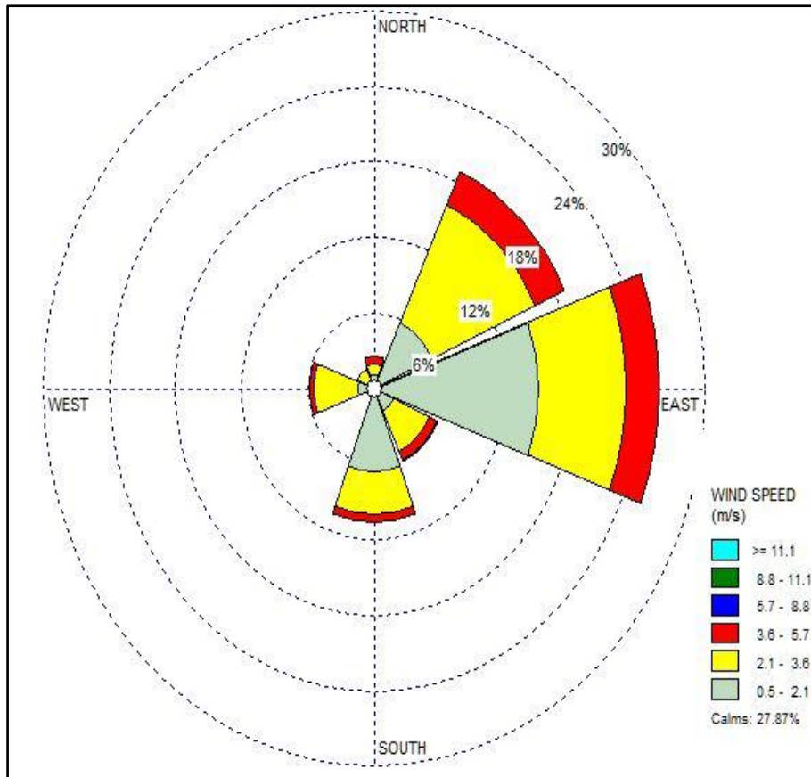
Figure 1-1 Wind rose diagram for the Study Period (October 2021-December 2021)
