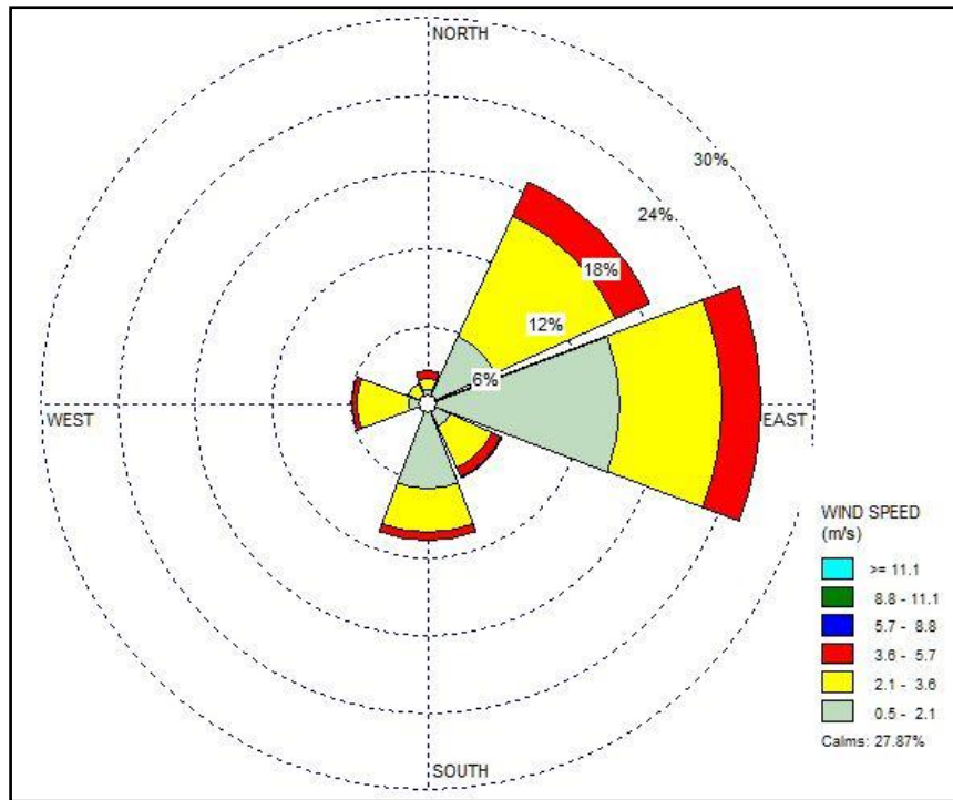
Figure Error! No text of specified style in document.-1 Wind rose diagram for the Study Period (October 2021-December 2021)
