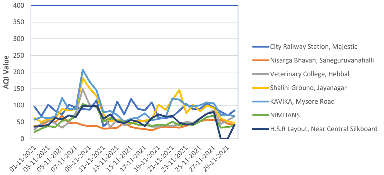
AQI Trend in CAAQMS, Bengaluru-2021
